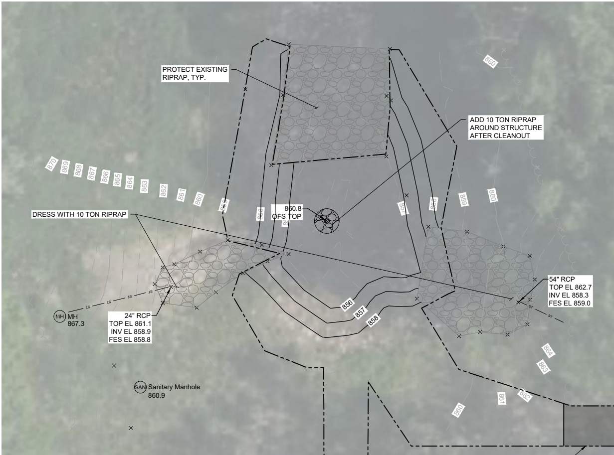
2 PLAN: BIRMINGHAM-YORK NORTH POND MAINTENANCE 0 10 20 SCALE IN FEET
