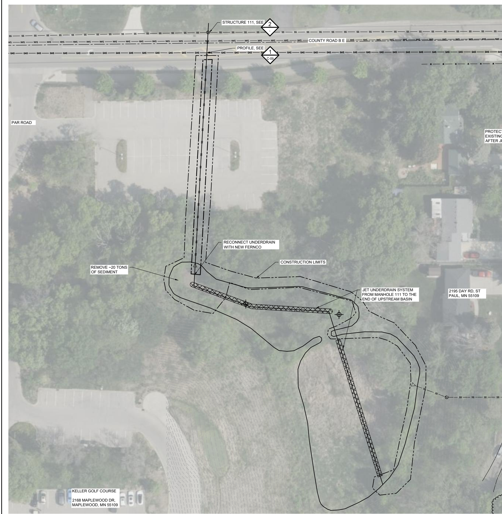
1 PLAN: DAY BASIN MAINTENANCE AND REPAIRS
