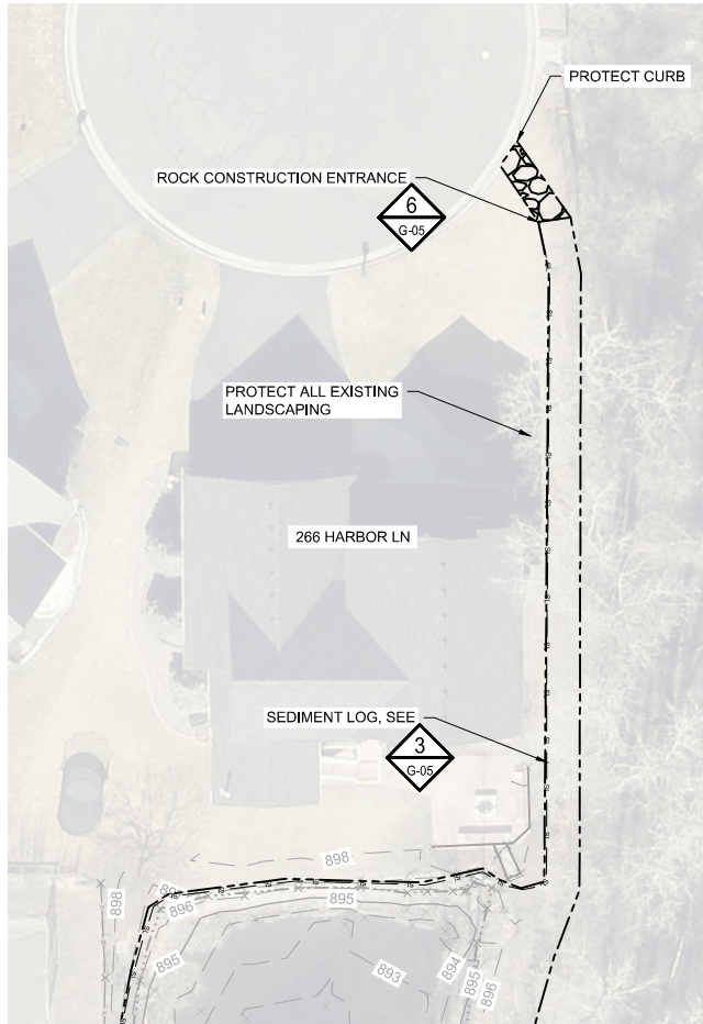
2 PLAN: HARBOR PLACE SOUTH ACCESS
