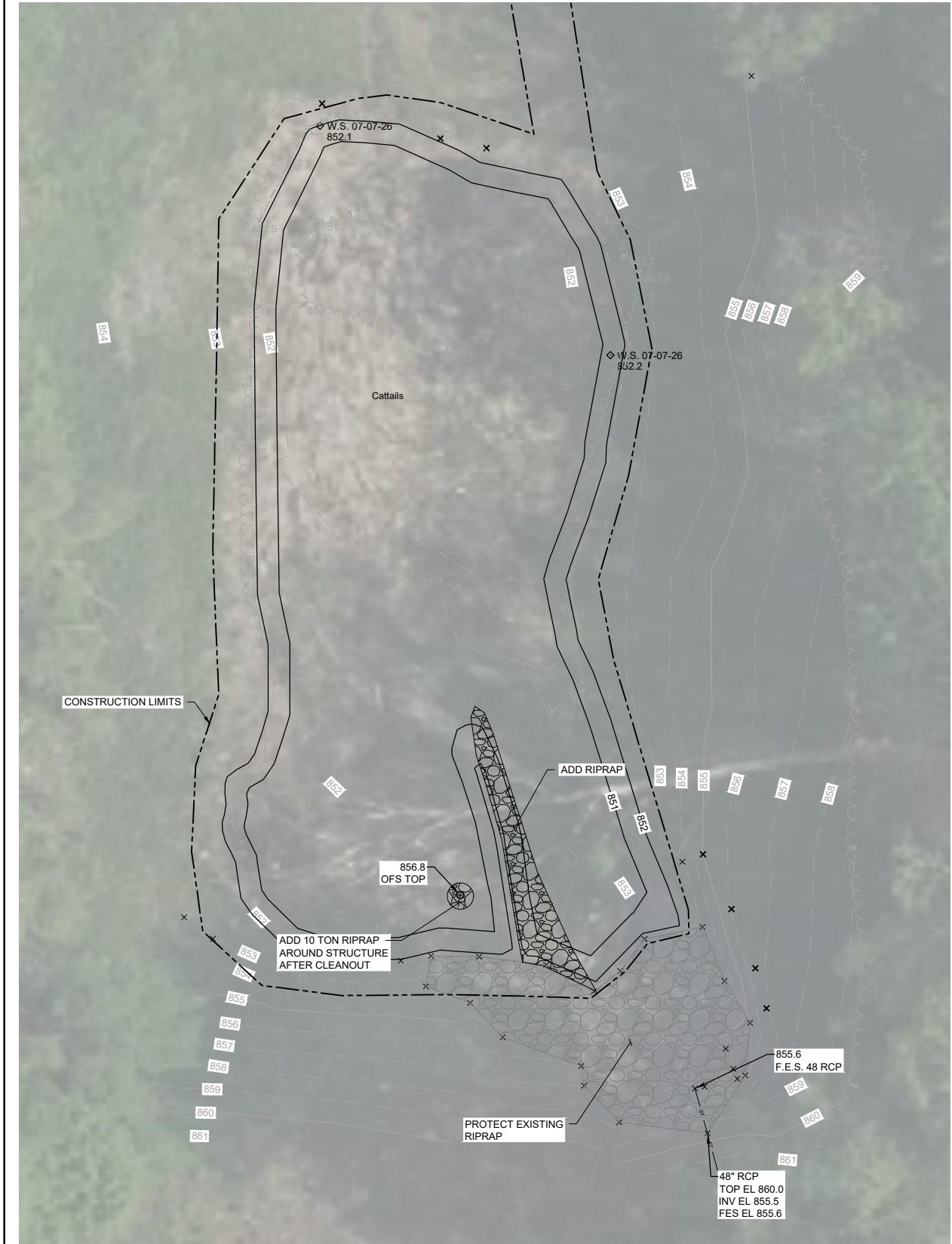
1 PLAN: BIRMINGHAM-YORK SOUTH POND MAINTENANCE 0 10 20 SCALE IN FEET
