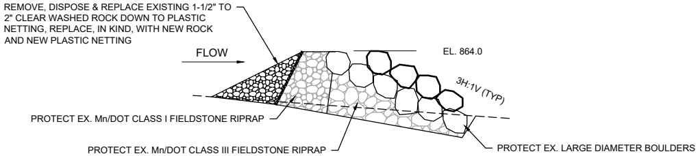
2 SECTION: EX. PERMANENT SEDIMENT CONTROL DIKE 0 4 8 SCALE IN FEET
