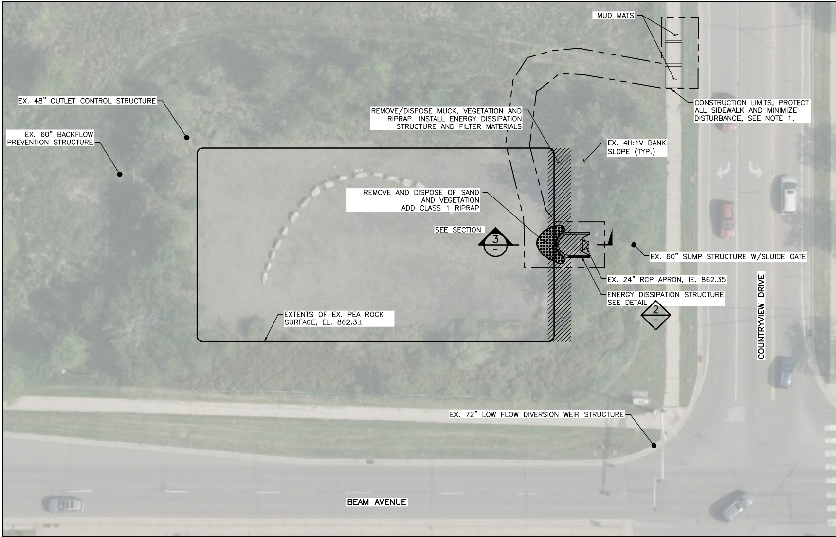
1 PLAN: KOHLMAN BASIN SAND FILTER INLET MODIFICATIONS
