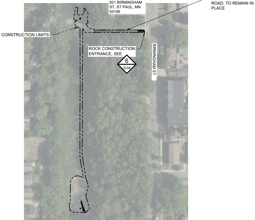
3 PLAN: CONSTRUCTION ACCESS 0 100 200 SCALE IN FEET
