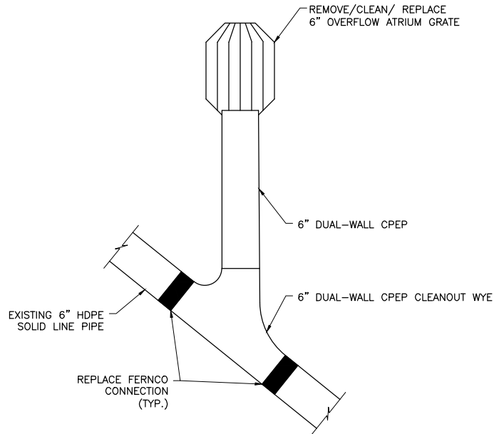
3 DETAIL: EXISTING INLINE CLEANOUT WYE, RISER W/ OVERFLOW GRATE NOT TO SCALE
