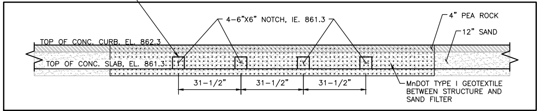
4 SECTION: DRAINAGE NOTCH OPENINGS
