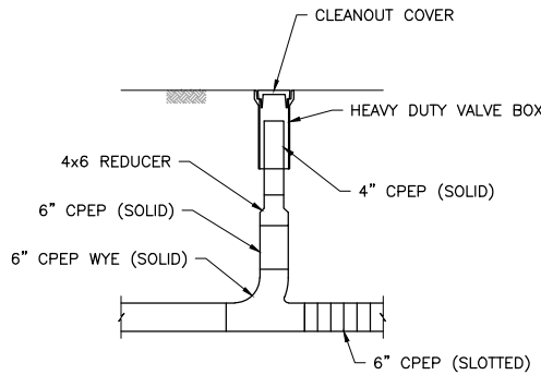
4 DETAIL: EXISTING DRAIN TILE SYSTEM - CLEAN OUT W/ WYE N.T.S.
