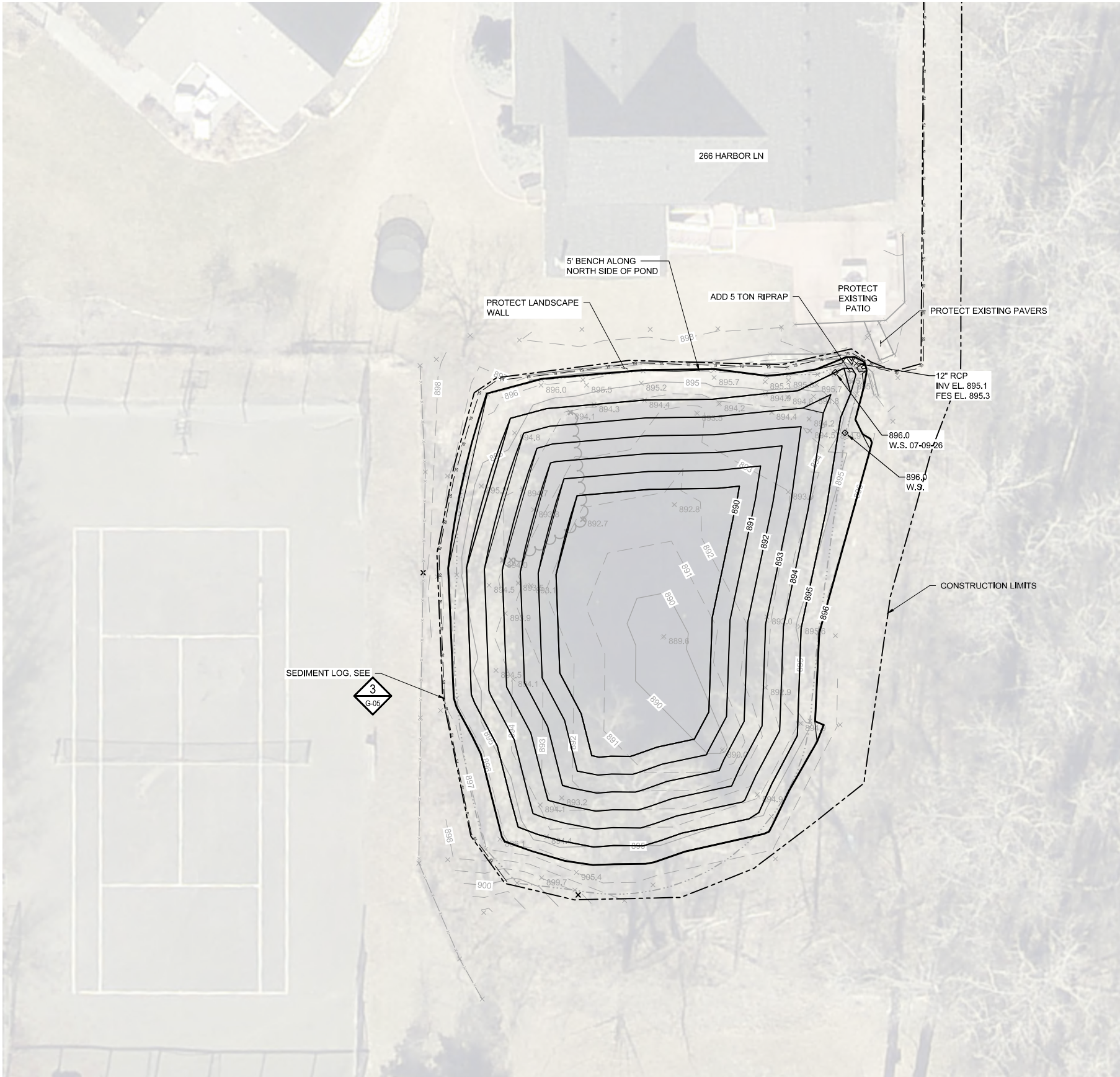
1 PLAN: HARBOR PLACE SOUTH MAINTENANCE
