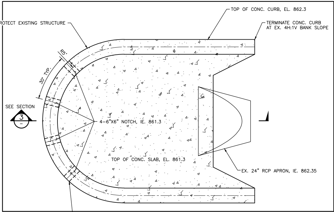
2 DETAIL: ENERGY DISSIPATION STRUCTURE
