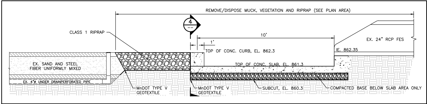
3 SECTION: ENERGY DISSIPATION STRUCTURE AND FILTER MODIFICATIONS
